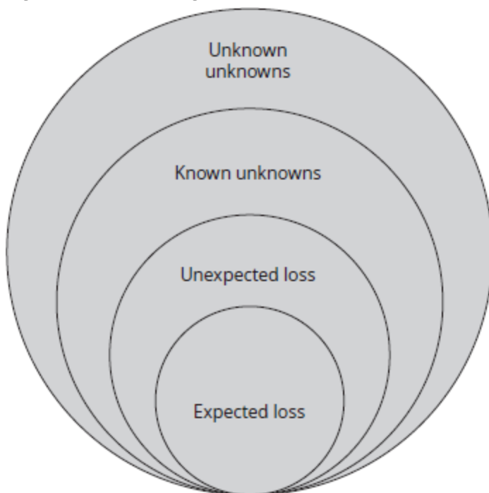
Figure 1.1: Loss Categories
